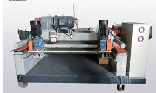
Single Power Spindleless Veneer Peeling Machine
