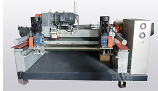
Single Power Spindleless Veneer Peeling Machine
